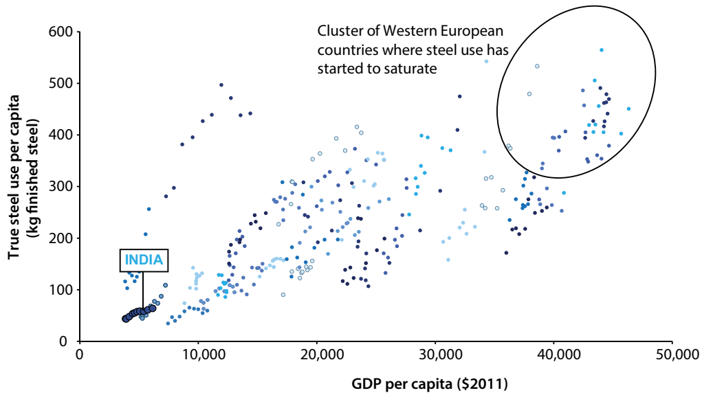
Figure 7: GDP per capita versus true steel use per capita for selected countries, 2006–16 Source: TERI analysis based on data from WSA (2018b); World Bank (2017)
