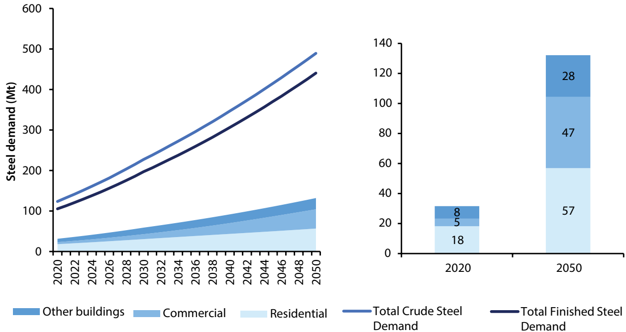
Figure 15: Projection of steel demand from buildings, 2020–50
