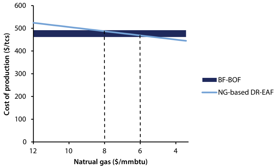
Figure 44: Costs of steel production from greenfield BF-BOF and gas-based DR-EAF plants at different natural gas prices
