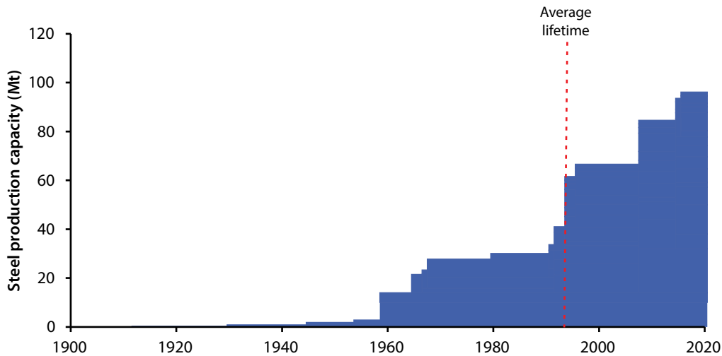
Figure 5: Production capacity of large steel plants by year of establishment Source: TERI analysis based on data from JPC (2018)
