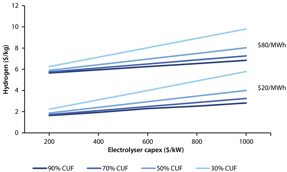
Figure 52: Impact of varying capacity utilization factors (CUF) on cost of hydrogen
