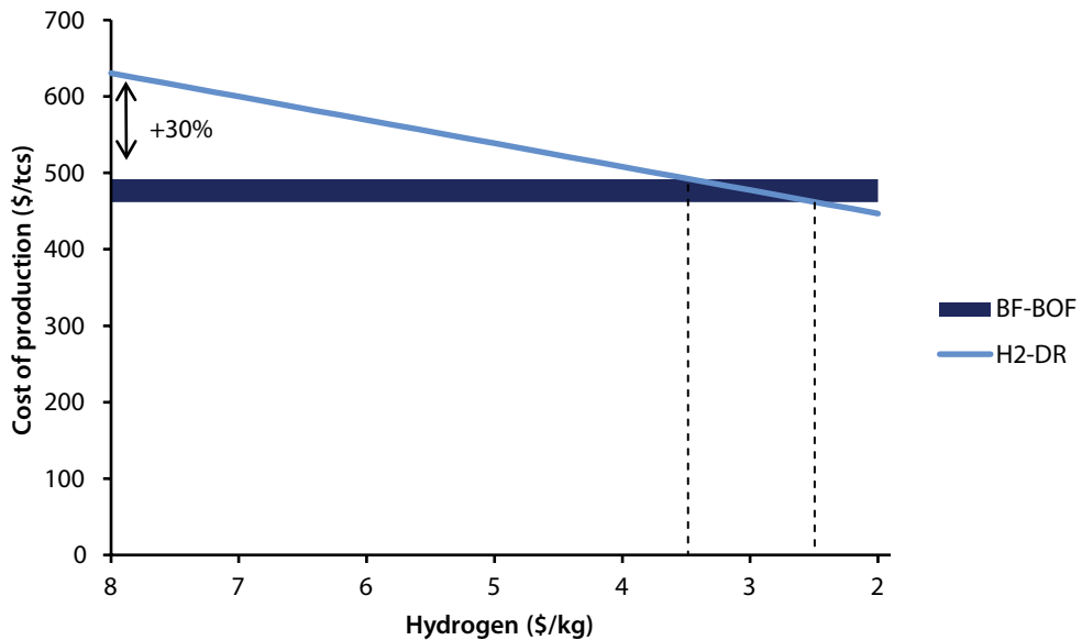
Figure 53: Cost of H2-DR versus BF-BOF for greenfield sites
