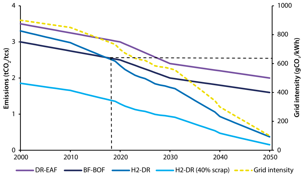
Figure 48: Emissions of different steelmaking routes
