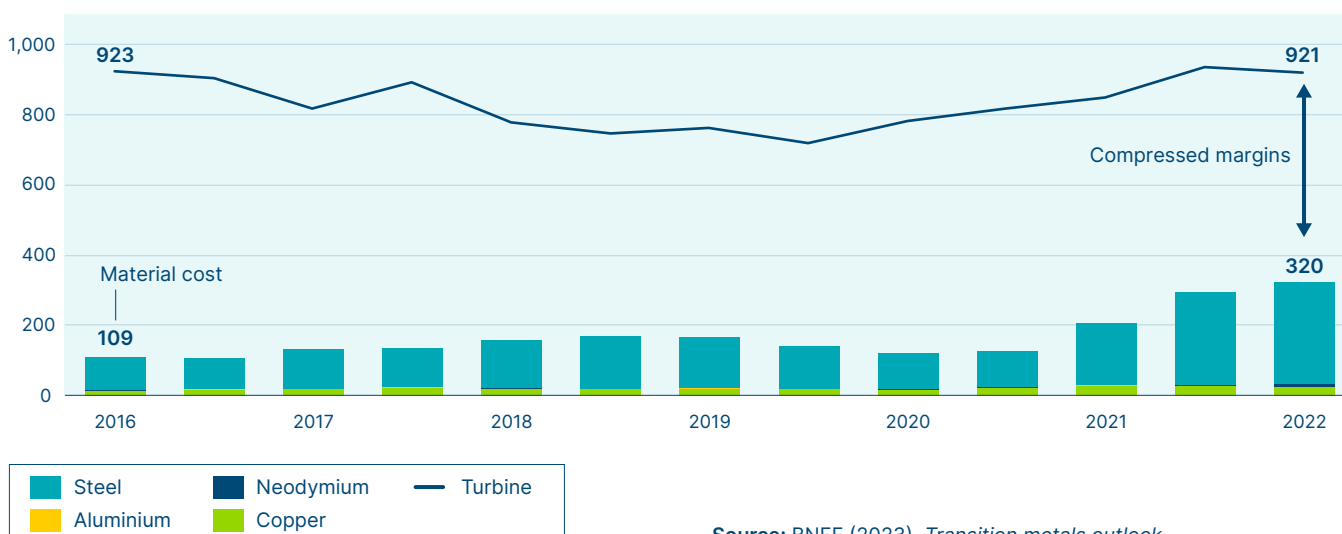
Metal and total wind turbine price Thousand $/MW
