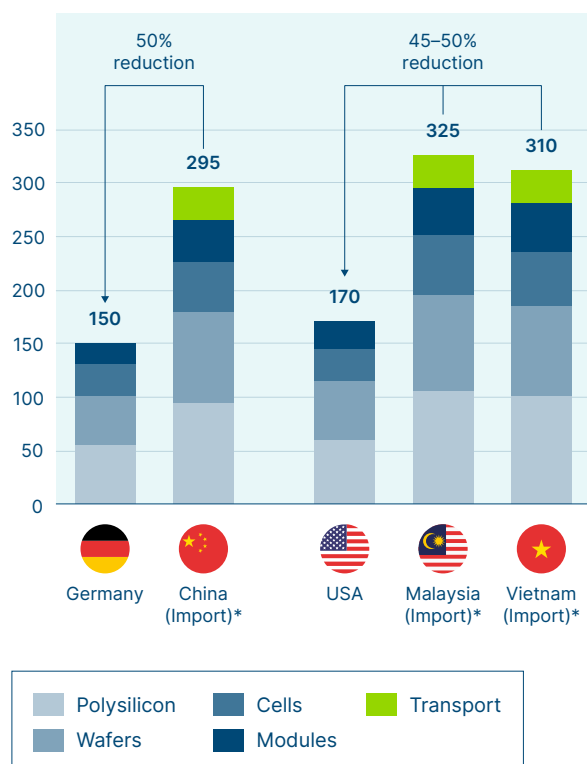
Module manufacturing emissions intensity tCO 2 e/MW
